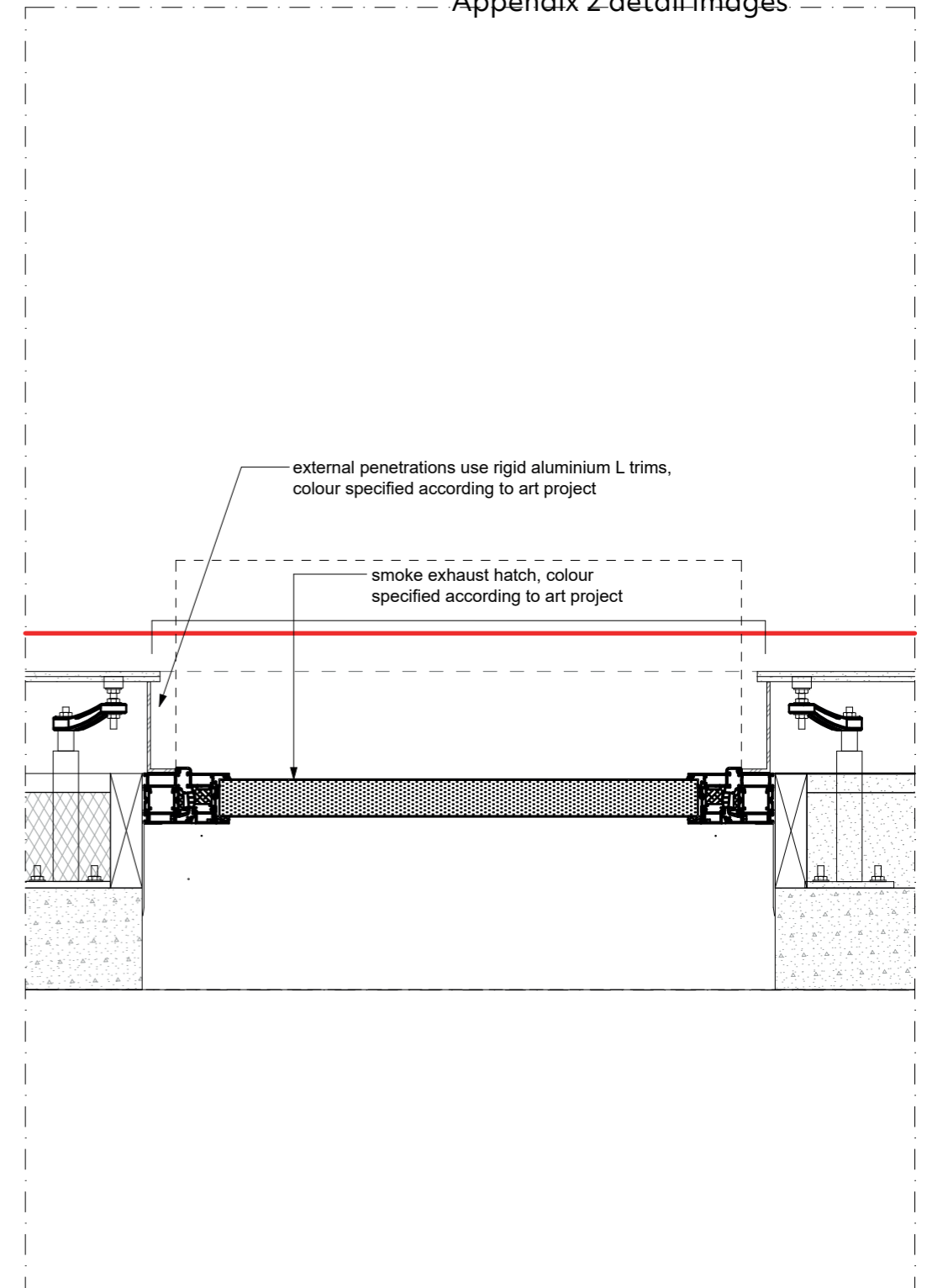
H.DET. 3 Smoke exhaust hatch 1:10
