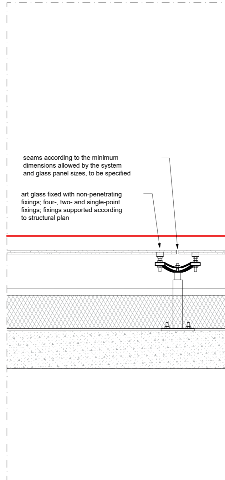
H.DET. 2 Glass panel joints 1:10
