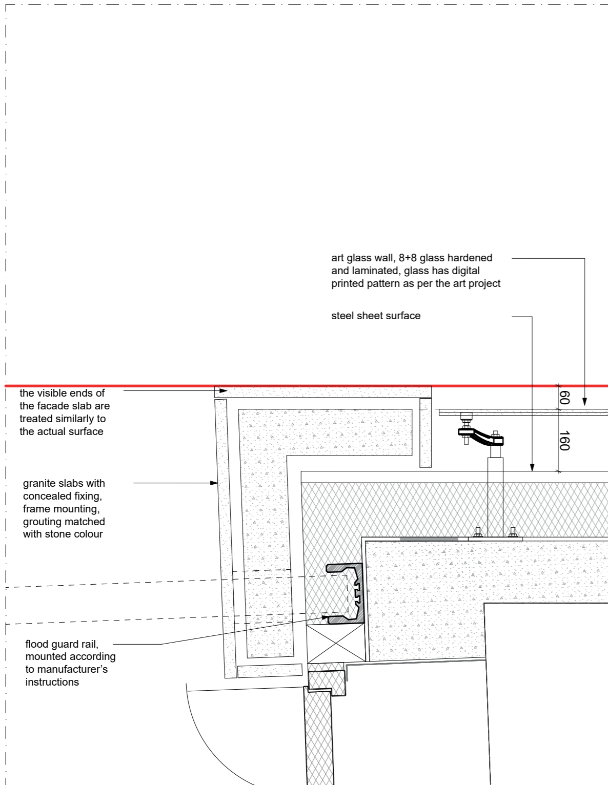
H.DET. 1 Fitting at a corner 1:10
